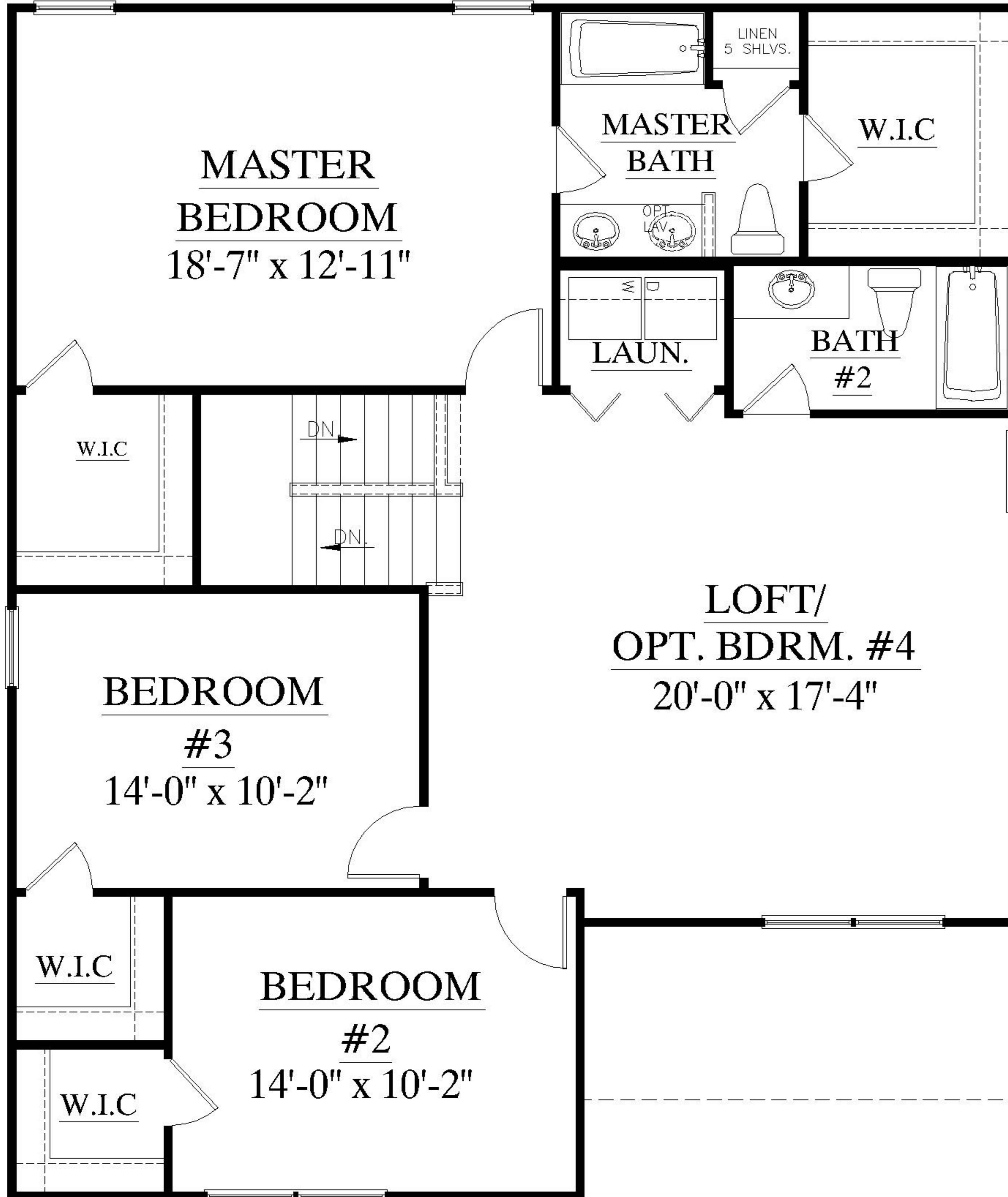
SECOND FLOOR PLAN
